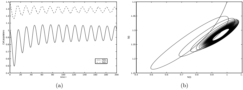
Figure 3: For \tau = 4.52 days, and the other parameters given by (34) with n = 12 , a Hopf bifurcation occurs and the steady state (S^*, N^*) of (3)–(4) is unstable. The periodic solutions S(t) (dashed line) and N(t) (solid line) are represented in (a), and we can observe the solutions in the (S, N) -plane in (b). Periods of the oscillations are about 15 days.
