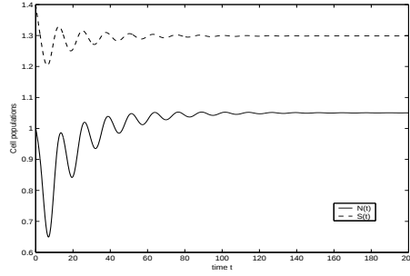
Figure 2: For \tau = 3.5 days, and the other parameters given by (34) with n = 12 , the solutions S(t) (dashed line) and N(t) (solid line) oscillate transiently to the steady state, which is asymptotically stable. Damped oscillations are observed.
