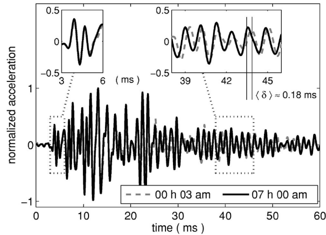
FIG. 8. Example of two dynamic responses at two different times: at midnight and at 7:00 a.m. The direct waves, i.e., the first ms of the records, do not change. Later in the coda, a slight delay d is observed. This delay is due to the weak thermal changes of the structure, resulting in an increase in the wave velocities. At night, the outside temperature is cold and the concrete structure is cooling down; therefore, the temperature at 12:03 a.m. is 3^{\circ}\text{C} lower than the one at 7:00 a.m. In this example, distortion, which changes the wave forms for varying temperature, is a very weak effect.
