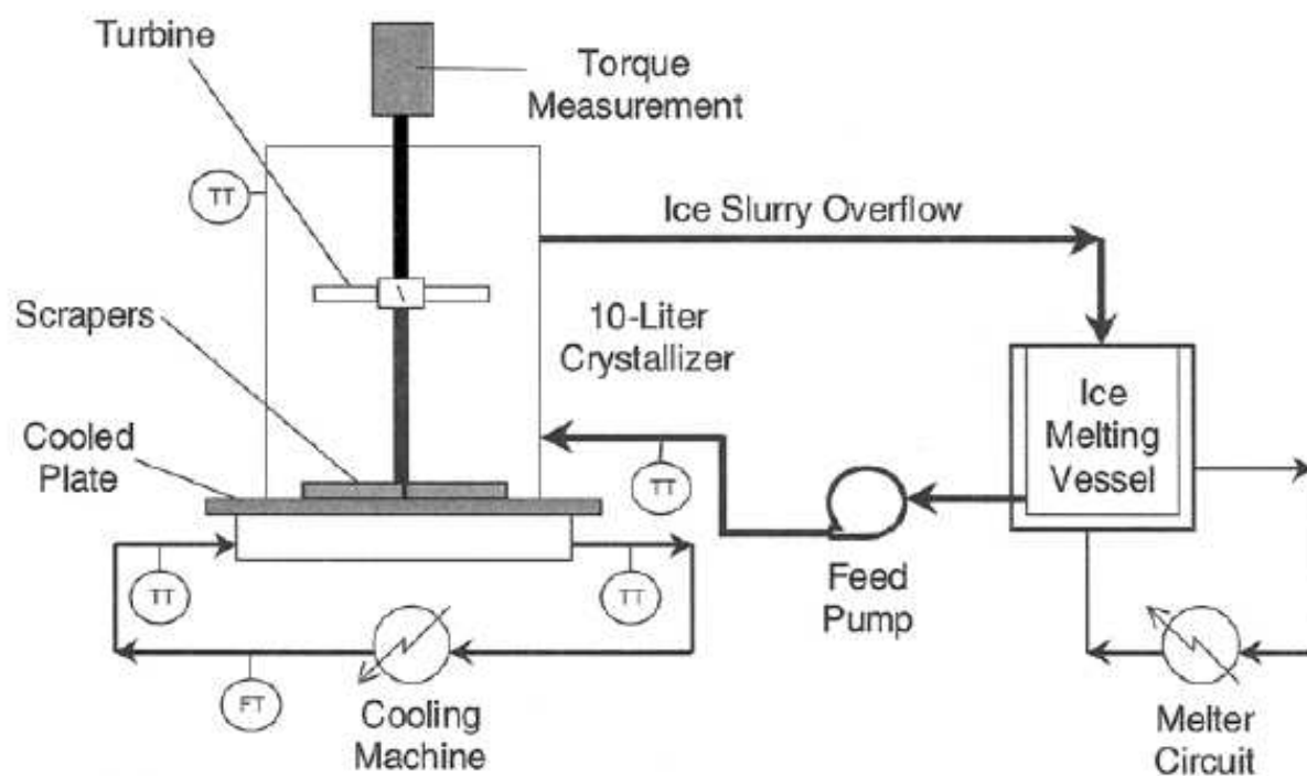
Figure1. Laboratory scale scraped cooling crystallizer. [Vassen et al.(2002)]
