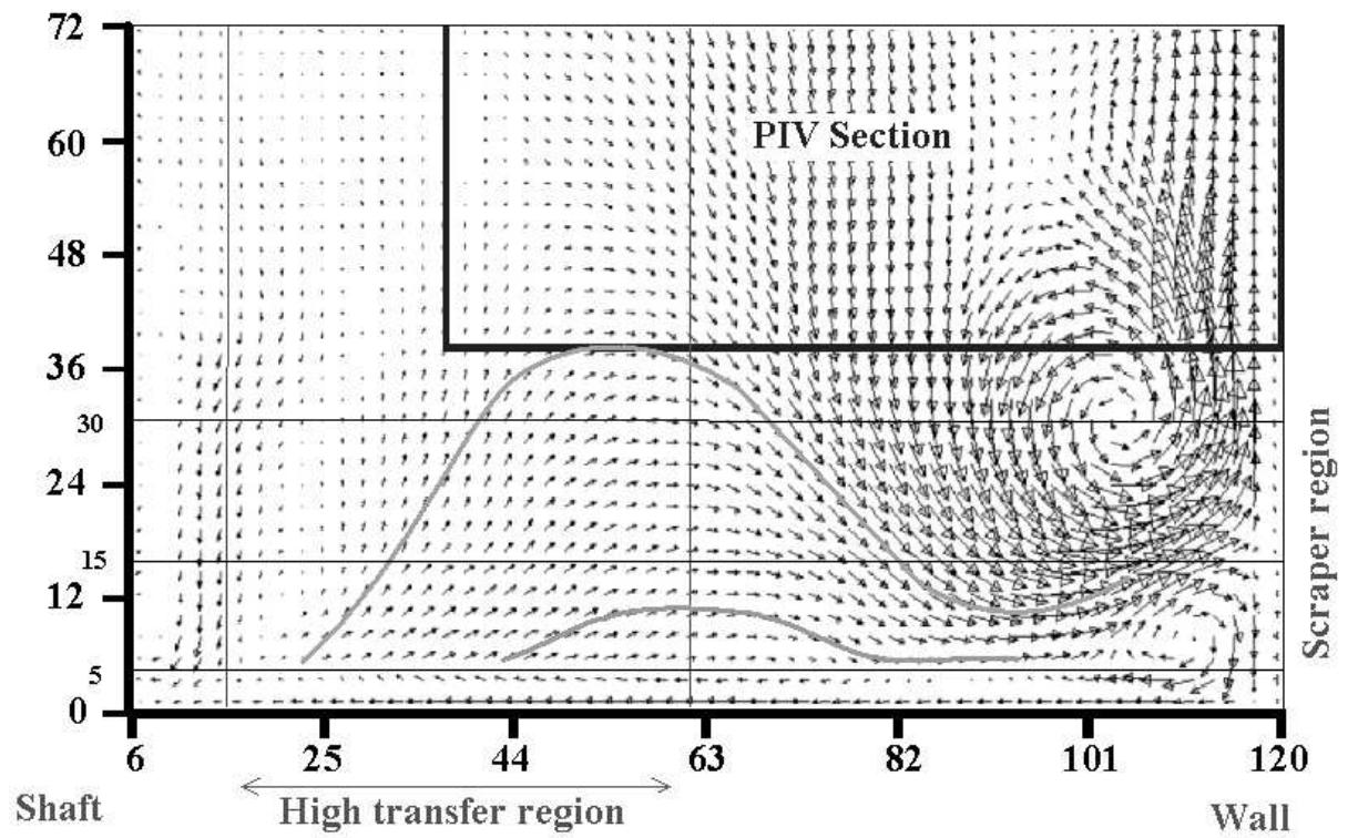
Figure 11. Axial-radial vector flow field area from the shaft to the wall and from the top of the 3C-PIV measured area to the scraped heat exchanger surface.
