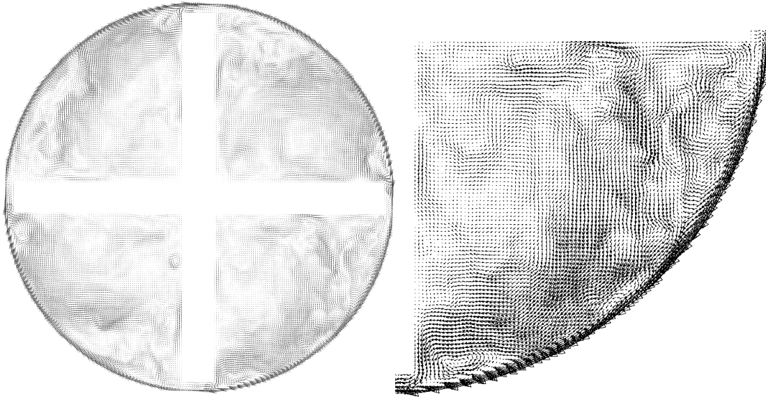
Figure 13. Instantaneous vertical view of the flow field in the frame of reference of the rotating scraper of the horizontal plane halfway the scraper height just above the HE and zoom of the right down quarter. The scraper rotates in the counter clockwise direction. In the rotating reference frame view of the figure, the wall now rotates clockwise.
