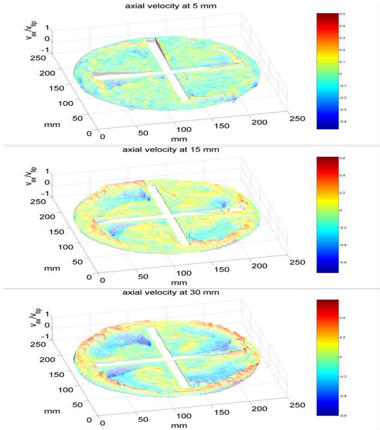
Figure 15. 3D surfaces of the instantaneous axial velocity at 5, 15 and 30 mm from the heat exchanger surface.
