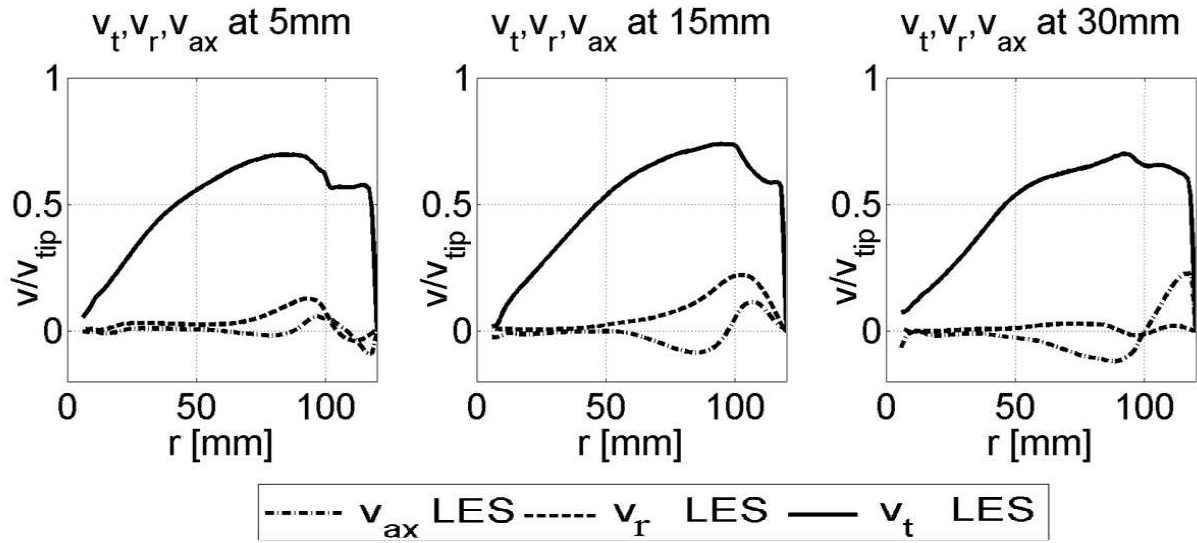
Figure 12. Time averaged tangential, radial and axial velocities calculated from LES simulations at heights of 5, 15 and 30 mm from the bottom plate in the scraper region.
