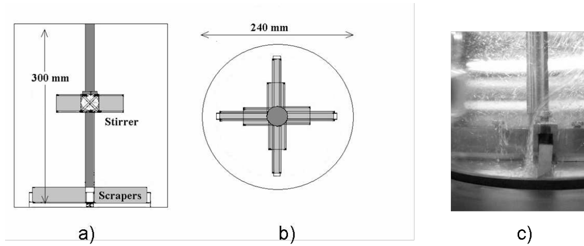
Figure 3a). Side view of the crystalliser. b). Top view of the crystalliser. c). Sideway view of the real scraper geometry.
