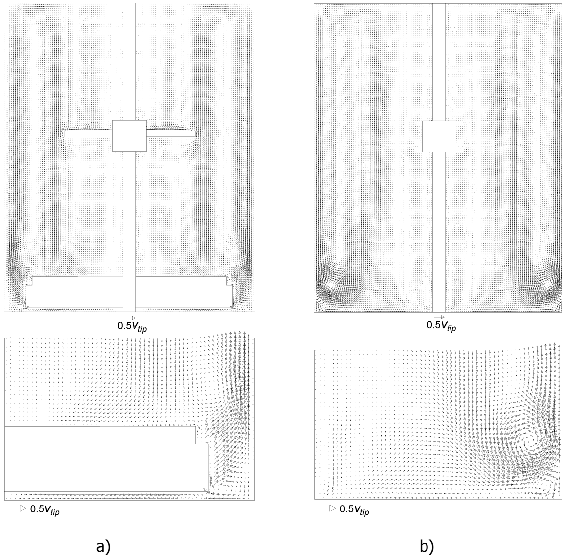
Figure 10. a) Time averaged flow field of the vertical cross section through the scrapers with an enlargement of the scraper area underneath. b) Time averaged flow field between the scrapers with an enlargement of the scraper area underneath.
