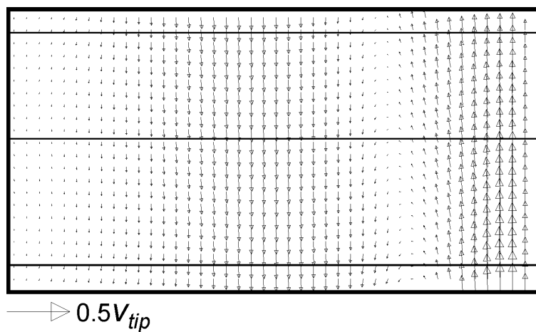
Figure 6. a) Time averaged velocity vectors of the flow field inside the scraped heat exchanger crystalliser. The black rectangle corresponds to the area measured by 3C-PIV. b) Computational results of the 3C-PIV measured area. The three lines across the measured area are drawn at heights of 45, 59 and 75 mm from the bottom plate.
