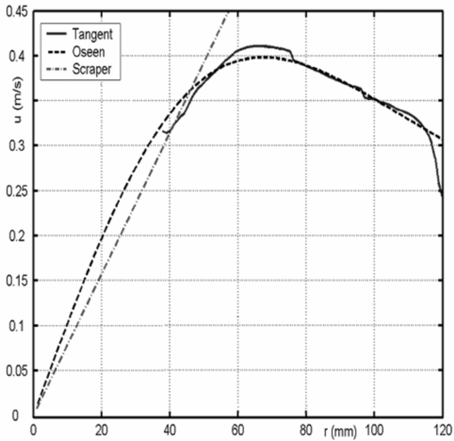
Figure 5. Measured time-axial averaged tangential velocity of the PIV area, the scraper velocity and the tangential velocity calculated from the Oseen approximation.
