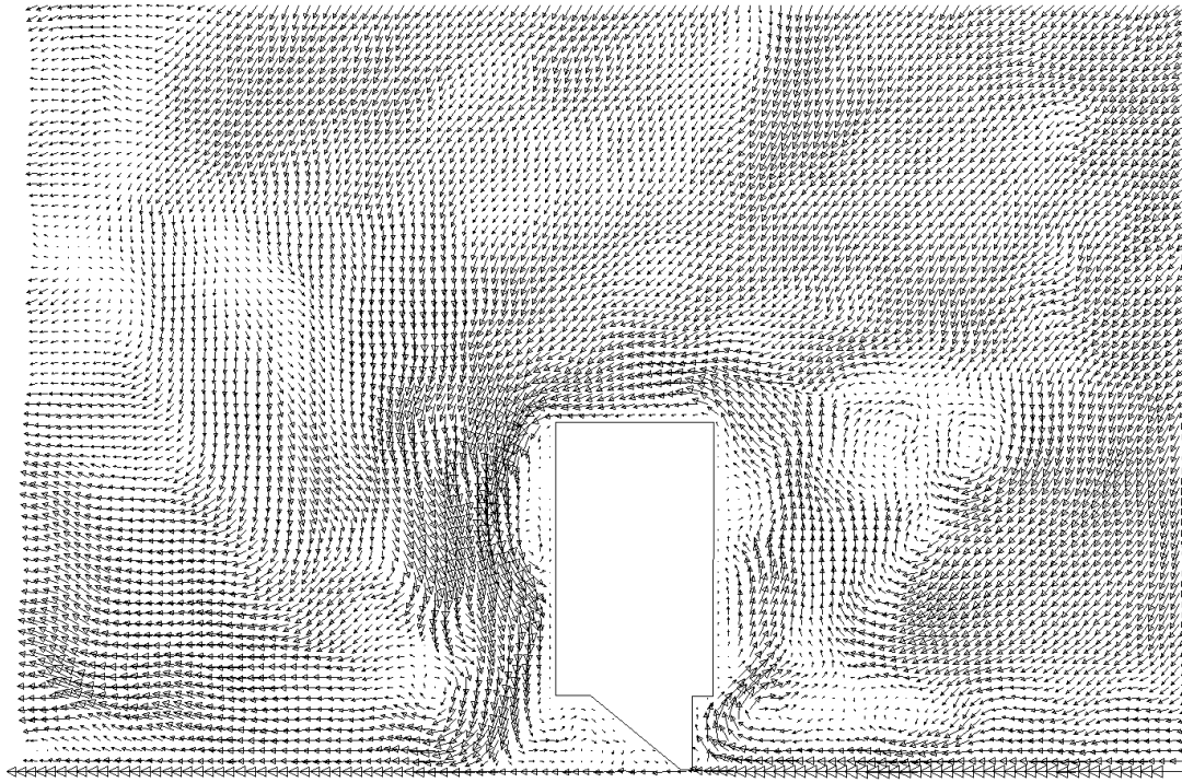
Figure 14. Instantaneous flow velocities of the vertical cut of the scraper region at the middle section of the scraper.
