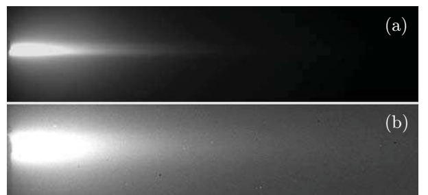
FIG. 2: Fluorescence images obtained after an exposure time of 30 minutes and dark frame subtraction, for (a) an incident laser beam at the atomic resonance frequency and (b) incident light provided by a first scattering cell. The temperature of the observation cell is 41°C. The step size distribution is extracted from the intensity along the axis.
