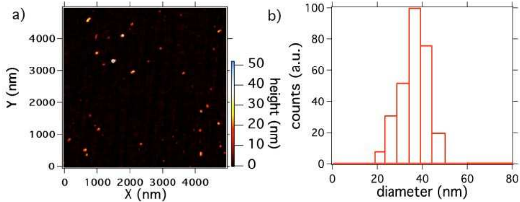
Figure 1: Size distribution of the PDNs (initial nanodiamond size < 50 nm) redispersed in the aqueous solution: a) Atomic Force Microscope scan of PDNs deposited on a mica plate (apparatus: Nanoscope IIIa , Veeco Instruments Inc., USA ). b) Dynamic Light Scattering measurement of PDNs in the aqueous solution (apparatus: BI-200SM , Brookhaven Instruments Corp., USA).
