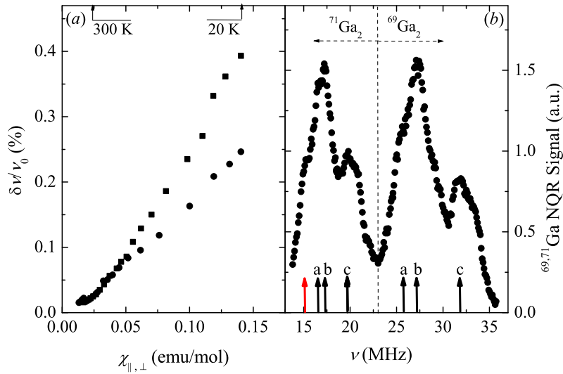
Figure 4. (a) Scaling of the relative line-width of the ^{29}\text{Si} NMR peak with susceptibility for \mathbf{H}||\mathbf{c} ( \bullet ) and for \mathbf{H} \perp \mathbf{c} ( \blacksquare ). (b) Ga NQR spectrum at 80 K, with thick black arrows indicating the position of three \text{Ga}_2 peaks (a, b, c) for each isotope and the red arrow the ^{69}\text{Ga}_3 peak.
