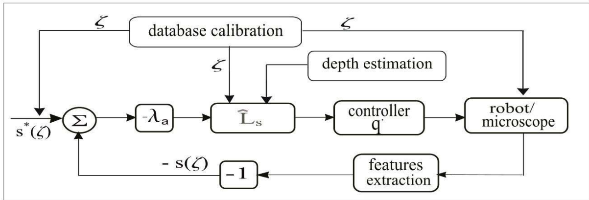
Fig. 1. The function chart of multiple scale image-based visual servoing
