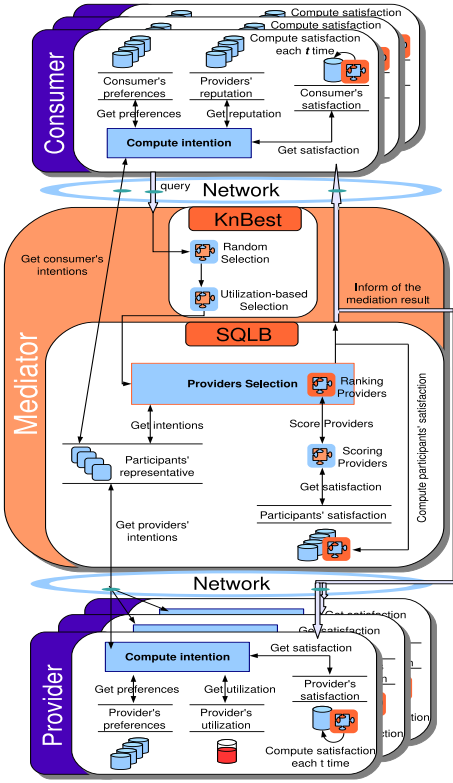
Fig. 1. System architecture.
