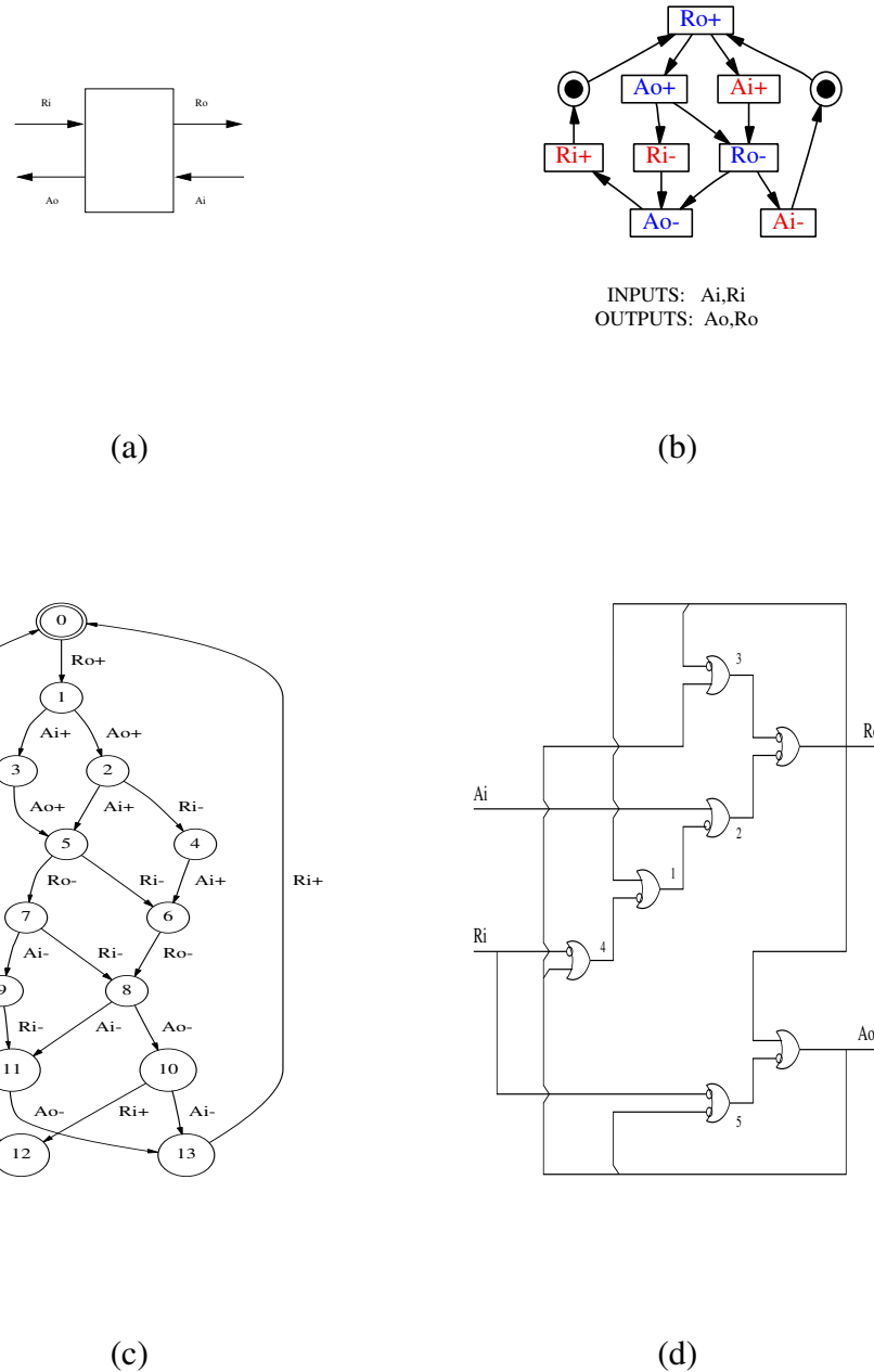
Fig. 5. The half circuit: (a) The block diagram. (b) The STG specification circuit. The boxes are PN transitions labeled by rising and falling of signals. All the PN places, except those with tokens at the initial configurations, are omitted. (c) The equivalent automaton for the specification. (d) The synthesized circuit.
