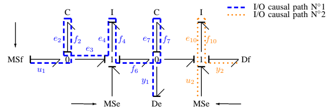
Fig. 4. Example of one set of two I/O causal paths
