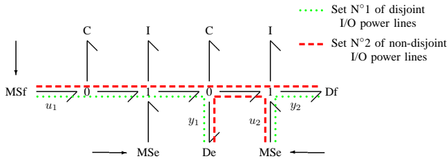
Fig. 2. Example of two sets of two I/O power lines
