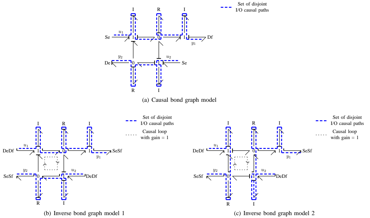
Fig. 5. Example of a model satisfying the two first conditions but which is not invertible
