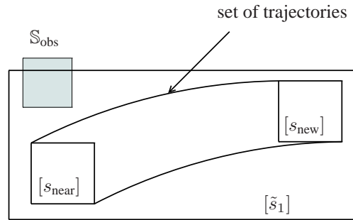
Fig. 2. The set of trajectories between [s_{\text{near}}] and [s_{\text{new}}] , wrapped in [\tilde{s}_1] , is reliable, but this cannot be proved, since [\tilde{s}_1] has a non-empty intersection with S_{\text{obs}} .
