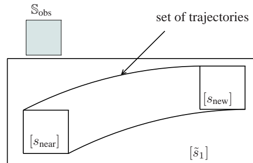
Fig. 3. The set of trajectories between [s_{\text{near}}] and [s_{\text{new}}] , wrapped in [\tilde{s}_1] , is proved to be reliable, since [\tilde{s}_1] has an empty intersection with \mathbb{S}_{\text{obs}} .
