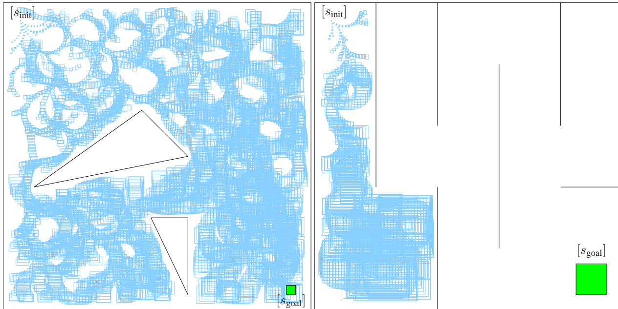
(a) Box-RRT fails to find a path (the goal area is too small)
