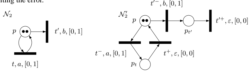
Fig. 5. A counter example to the construction of [4].
