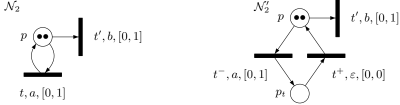
Fig. 5. A counter example to the construction of [4].
