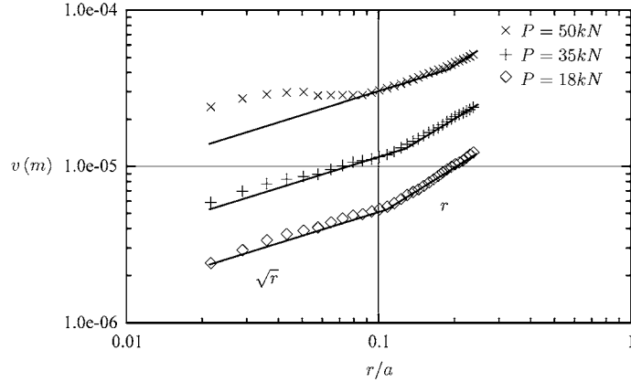
Figure 8. Vertical displacement and power law approximations.
