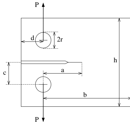
Figure 4. Geometry of the compact tension specimen.
