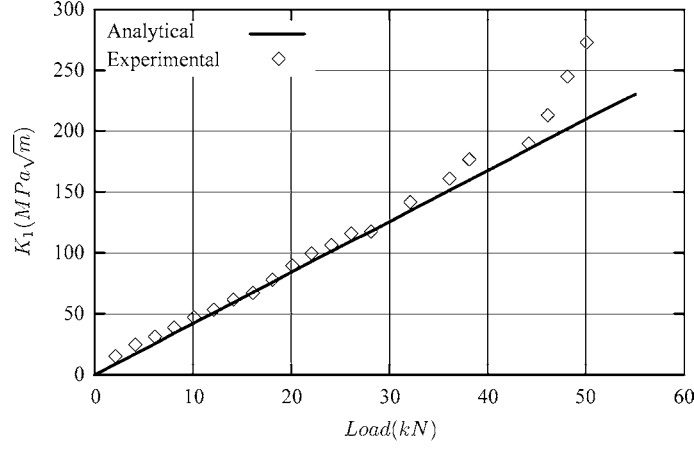
Figure 6. Comparison of analytical and experimental values of K_I .
