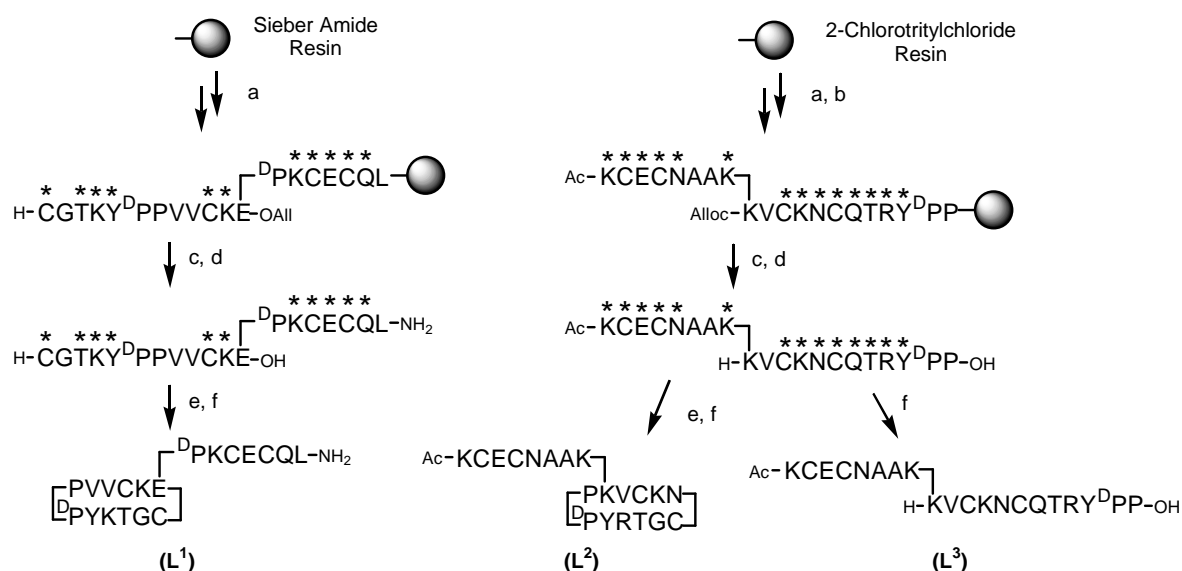
Scheme 1. Synthesis of peptides L i . (a) Fmoc SPPS; (b) DMF/pyridine/Ac 2 O 7:2:1; (c) Pd(PPh 3 ) 4 , PhSiH 3 , CH 2 Cl 2 ; (d) CH 2 Cl 2 /TFA 99:1; (e) 0.25 mM, PyBOP, DIEA, CH 2 Cl 2 ; (f) TFA/TIS/H 2 O/DTT. * denotes side-chain protecting groups.
