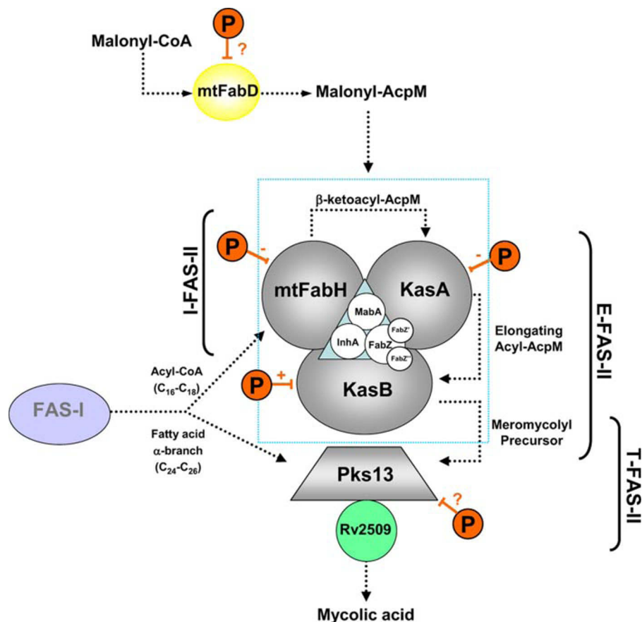
FIGURE 7. Proposed regulatory role of condensase phosphorylation in mycolic acid initiation, elongation and termination. Mycolic acid biosynthesis is initiated via de novo biosynthesis of C_{16-26} -CoA by the mycobacterial FAS-I and further extended to the meromycolate precursor by FAS-II. FAS-I provides both the initiation primer ( C_{16} -CoA) for FAS-II and the C_{24-26} fatty acid utilized by the Claisen-type condensing enzyme Pks13 (belonging to the T-FAS-II system) during the formation of the nonreduced mycolic acid. The initiation primer is utilized by mtFabH (a feature of the I-FAS-II system), forming a \beta -ketoacyl-AcpM product, which is further modified via the reductive cycle of FAS-II performed by MabA, FabZ, FabZ', and InhA. The derived aliphatic acyl-AcpM then is used as the substrate of the condensing enzymes KasA and KasB of the E-FAS-II systems. KasA is involved in the elongation of the meromycolate precursors that are further extended to their full lengths by KasB. The condensing enzymes are shown in gray. Experimental evidence has demonstrated phosphorylation of all four condensases. Phosphorylation can either activate (+) or inhibit (-) the condensing activity. A question mark indicates that the effect of phosphorylation on the enzyme activity has not yet been investigated.
