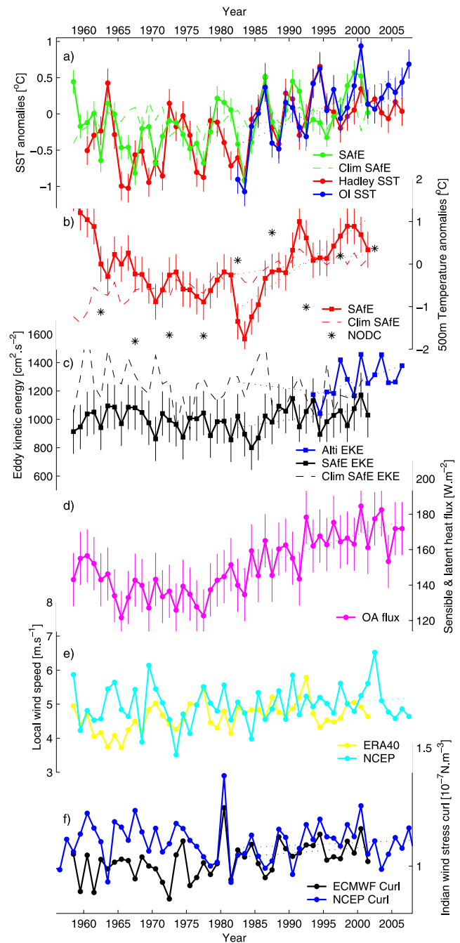
Figure 2. Changes in the Agulhas Retroflexion region ( 36^{\circ}\text{S} to 41^{\circ}\text{S} and 10^{\circ}\text{E} to 20^{\circ}\text{E} ) from 1960 to 2006. Dashed lines represent a model run forced by monthly climatology. Interannual variability RMSs in this climatological simulation are used as model error bars. (a) Observed (red and blue + error bars: \pm 0.2^{\circ}\text{C} ) and modeled (green) SST anomalies [ ^{\circ}\text{C} ]. (b) Modeled (red) and observed (black stars) temperature anomalies [ ^{\circ}\text{C} ] at 500 m. (c) Modeled (black) and observed (blue) geostrophic eddy kinetic energy [ \text{cm}^2/\text{s}^2 ] derived from sea surface height. (d) Observed latent plus sensible heat fluxes (purple) [ \text{W.m}^{-2} ] and error bars ( \pm 15 \text{ W.m}^{-2} ). (e) ERA 40 (yellow) and NCEP (cyan) surface wind speed [ \text{m.s}^{-1} ]. (f) Wind stress curl [ 10^{-7} \text{N.m}^{-3} ] calculated from NCEP (blue) and from ERA40 (black) for the whole South Indian Ocean ( 20^{\circ}\text{S} to 40^{\circ}\text{S} and 50^{\circ}\text{E} to 100^{\circ}\text{E} ). Dotted lines are linear fits to data from 1980 onwards.
