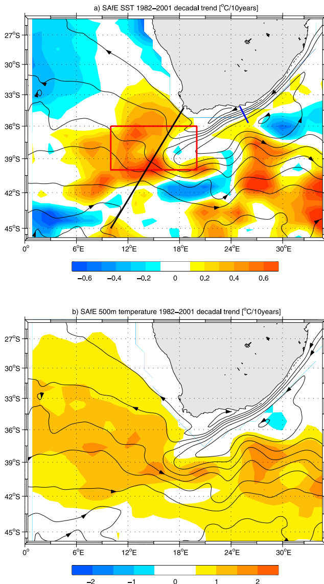
Figure 3. Modeling the recent warming in the Agulhas Current system. (a) Linear trend in modeled SST from 1982 to 2001 [°C/decade]. (b) Linear trend in modeled temperature [°C/decade] at 500 m for the same period. The black contours represent the model sea surface elevation (1 contour per 20cm) accounting for the mean surface currents for the same period. Arrows indicate the direction of the flow.
