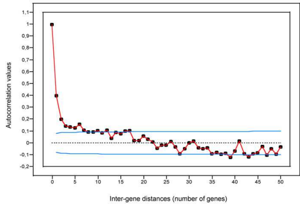
Figure 4 Autocorrelation function of the spatial series corresponding to the Buchnera \log_2 nBGT along the chromosome. The blue lines represent \pm 2 standard errors for approximate 95% confidence limits (i.e., values above the threshold are significant).
