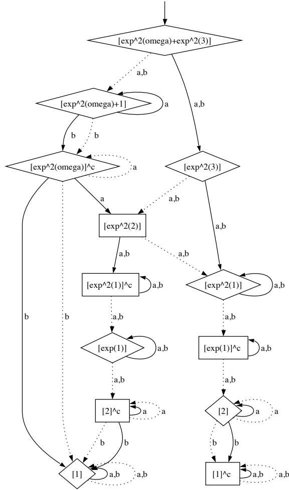
Fig. 4. ... and the computation of its Wadge degree.
