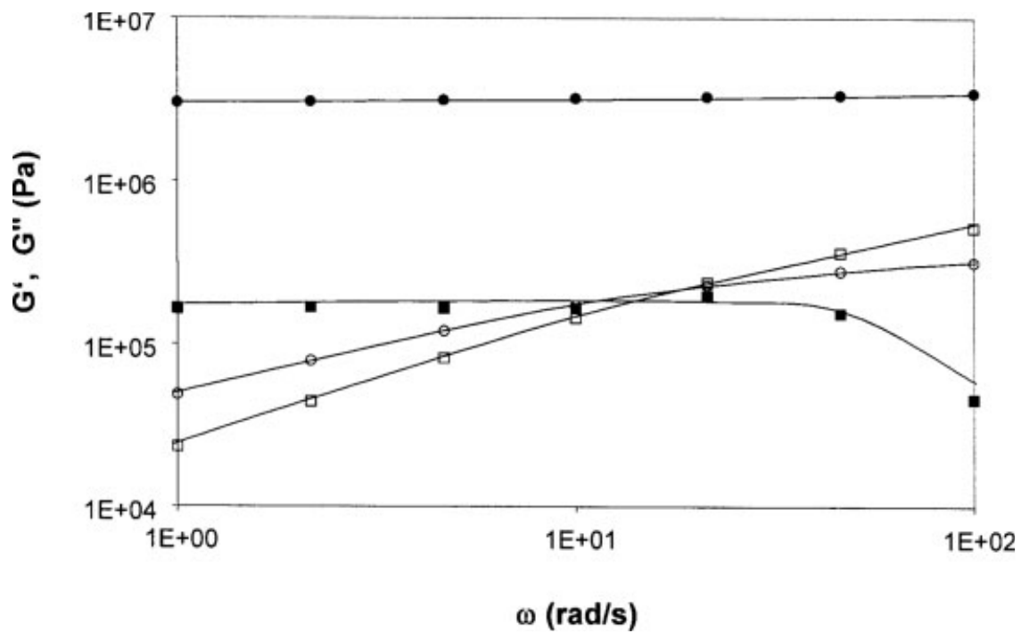
Figure 10. Plot of (●,○) G' and (■,□) G'' as functions of the oscillation frequency ( \omega ) at the beginning and end of an annealing step ( T_a = 110^\circ\text{C} ) for the pristine TPU [ \varepsilon = 0.45 ; thermal treatment: T^* = 220^\circ\text{C} , t^* = 3 min, -q = 50^\circ\text{C}/\text{min} , and t_a = 0 (○,□) or 166 min (●,■)].
