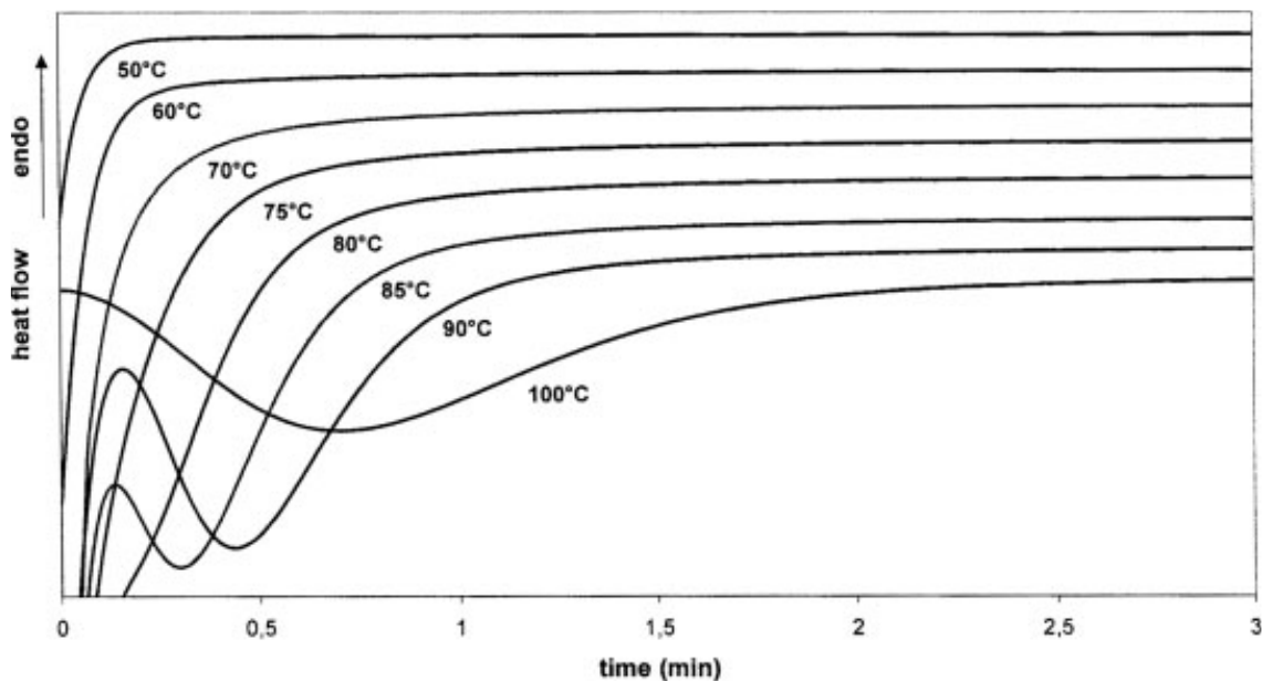
Figure 5. DSC isothermal traces of the TPUs during annealing at different T_a 's. The thermal treatment was as follows: T^* = 220^\circ\text{C} , t^* = 3 min, -q = 50^\circ\text{C}/\text{min} , T_a = 50\text{--}100^\circ\text{C} , and t_a = 15 min. Only the first 3 min are represented here.
