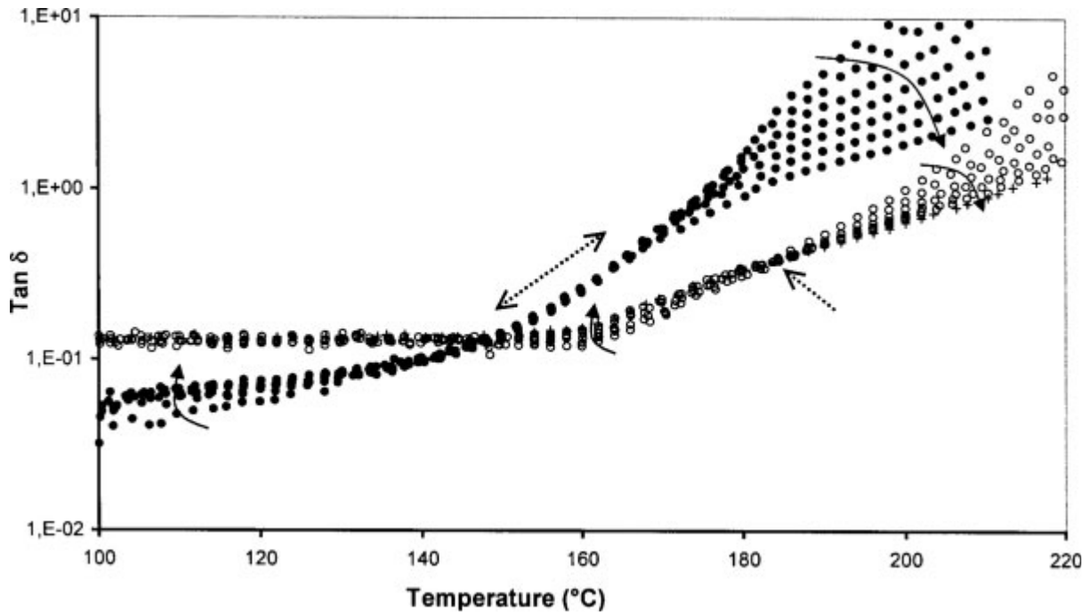
Figure 15. \tan \delta as a function of the temperature for the initial TPU and the MDI-modified TPU. The thermal treatment was as follows: T^* = 220^\circ\text{C} , t^* = 3 min, -q = 50^\circ\text{C}/\text{min} , T_a = 80^\circ\text{C} , t_a = 15 min, and +q = 0.5^\circ\text{C}/\text{min} . The gel content of the modified TPU was 15% during the annealing. The measurements were recorded at different oscillation frequencies between 1 and 100 rad/s. The bent arrows indicate that the oscillation frequency increases. The dotted arrows indicate the \tan \delta crossings. The filled symbols correspond to the initial TPU, and the open symbols correspond to the MDI-modified TPU.
