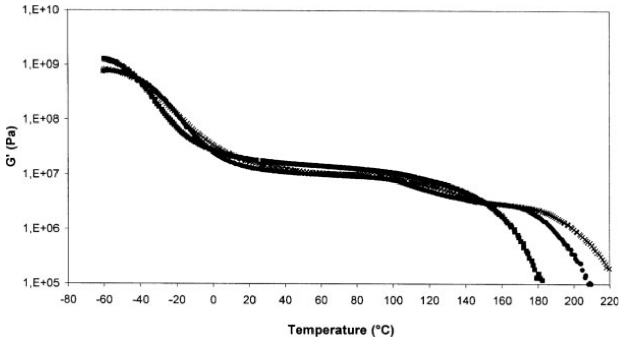
Figure 16. Evolution of G' as a function of the temperature: (■) the initial TPU, (●) the MDI-modified TPU (isocyanate/urethane ratio (i/u) = 0.107), and (×) the tIPDI-modified TPU (isocyanate/urethane ratio (i/u) = 0.055).
