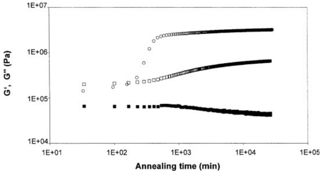
Figure 11. Evolution of G' and G'' during annealing ( T_a = 110^\circ\text{C} , T^* = 220^\circ\text{C} , t^* = 3 min, -q = 50^\circ\text{C}/\text{min} , \varepsilon = 0.45 , and \omega = 10 rad/s): (○) G' for the initial TPU, (□) G' for the 15-gelled TPU, and (■) G'' for the 15-gelled TPU.
