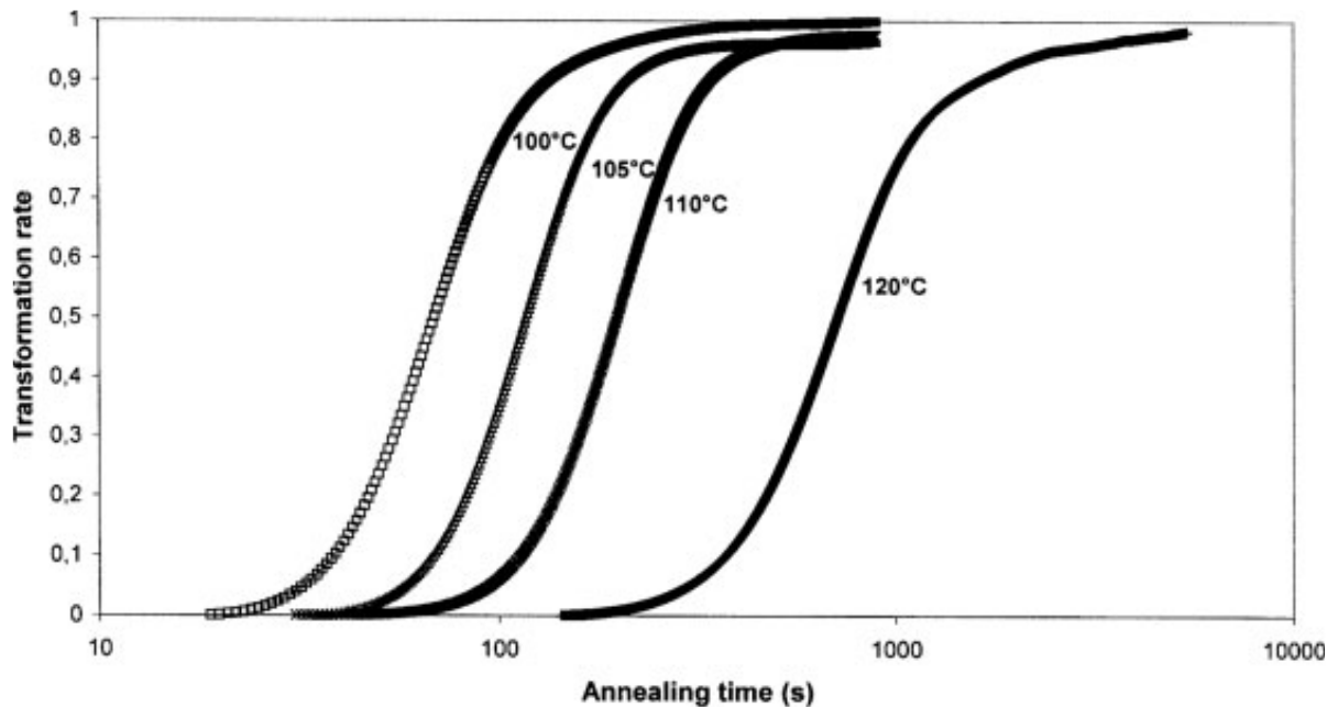
Figure 6. Transformation rate ( \Delta H_t/\Delta H_{max} ) for the initial TPU as a function of t_a and T_a . The thermal treatment was as follows: initial gel content = 100%, T^* = 220^\circ\text{C} , t^* = 3 min, -q = 50^\circ\text{C}/\text{min} , gel content during the annealing = 15%, and T_a = 100\text{--}120^\circ\text{C} .
