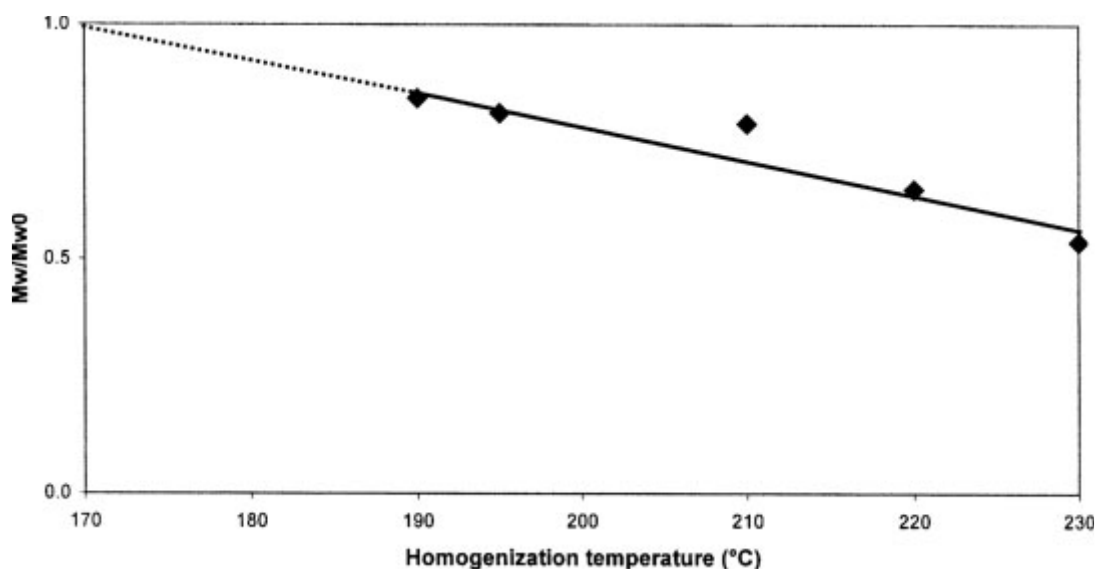
Figure 4. M_w/M_{w0} ratio as a function of T^* . M_w is the molar mass of TPUs held at T^* for time t^* , and M_{w0} is the molar mass of the initial TPU. The thermal treatment was as follows: T^* = 190\text{--}230^\circ\text{C} , t^* = 3 min, -q = 50^\circ\text{C}/\text{min} , and t_a = 0 min.
