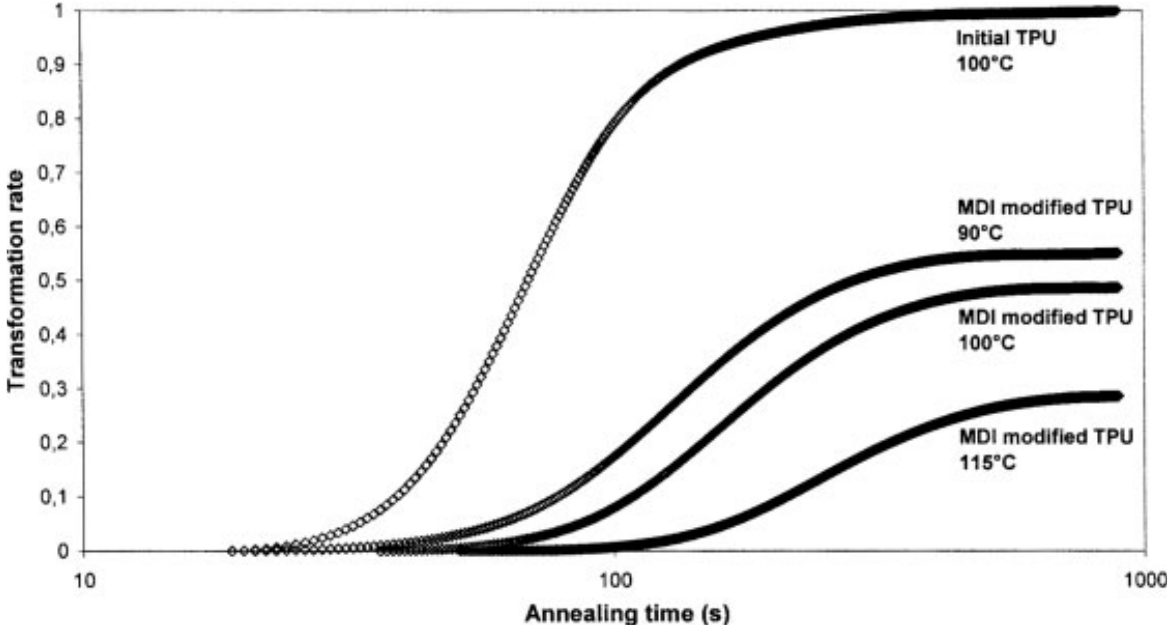
Figure 7. Transformation rate ( \Delta H_t/\Delta H_{max} ) for the initial TPU and the MDI-modified TPU as a function of t_a for different T_a 's. The thermal treatment was as follows: initial gel content = 100%, T^* = 220^\circ\text{C} , t^* = 3 \text{ min} , -q = 50^\circ\text{C}/\text{min} , gel content during the annealing = 15%, and T_a = 90\text{--}115^\circ\text{C} .
