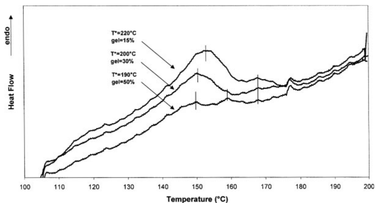
Figure 14. DSC thermograms obtained for MDI-modified TPU. The thermal treatment was as follows: T^* = 190\text{--}220^\circ\text{C} , t^* = 3 min, -q = 50^\circ\text{C}/\text{min} , T_a = 100^\circ\text{C} , t_a = 15 min, and +q = 10^\circ\text{C}/\text{min} . The T^* values and the resulting gel contents of the sample are indicated.
