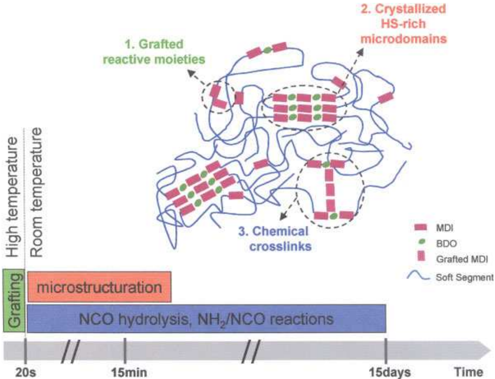
Figure 8. Schematic representation of the different elements present in the MDI-modified TPU microstructure and possible schedule of the successive events leading to their formation.
