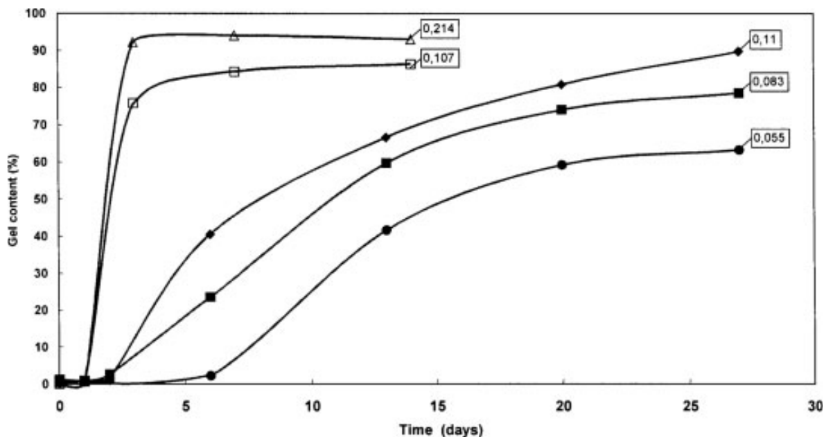
Figure 2. Evolution of the gel content at room temperature for TPUs modified by MDI and by tIPDI in a twin-screw extruder and reprocessed with a single-screw extruder. The filled symbols correspond to the tIPDI-modified TPU, and the open symbols correspond to the MDI-modified TPU. The isocyanate-to-urethane ratio is indicated for each species.
