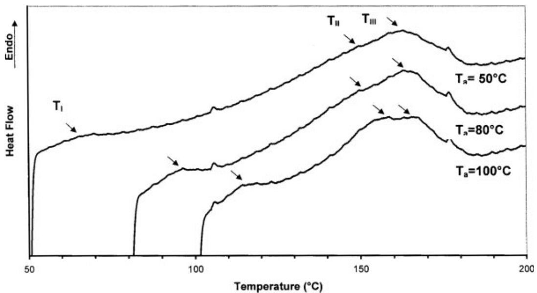
Figure 12. DSC thermograms obtained for unmodified TPU samples. The thermal treatment was as follows: T^* = 220^\circ\text{C} , t^* = 3 min, -q = 50^\circ\text{C}/\text{min} , T_a = 50\text{--}100^\circ\text{C} , t_a = 15 min, and +q = 10^\circ\text{C}/\text{min} .
