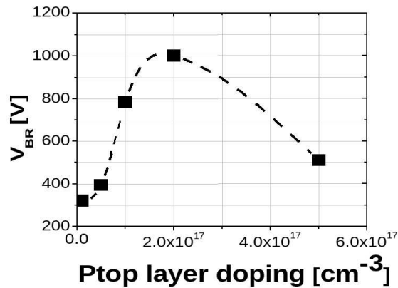
Fig. 16. V_{BR} versus top layer doping for the JFET structure.
