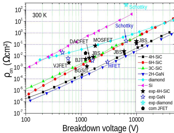
Fig. 1. On state resistance for unipolar devices for various semiconductor materials.
