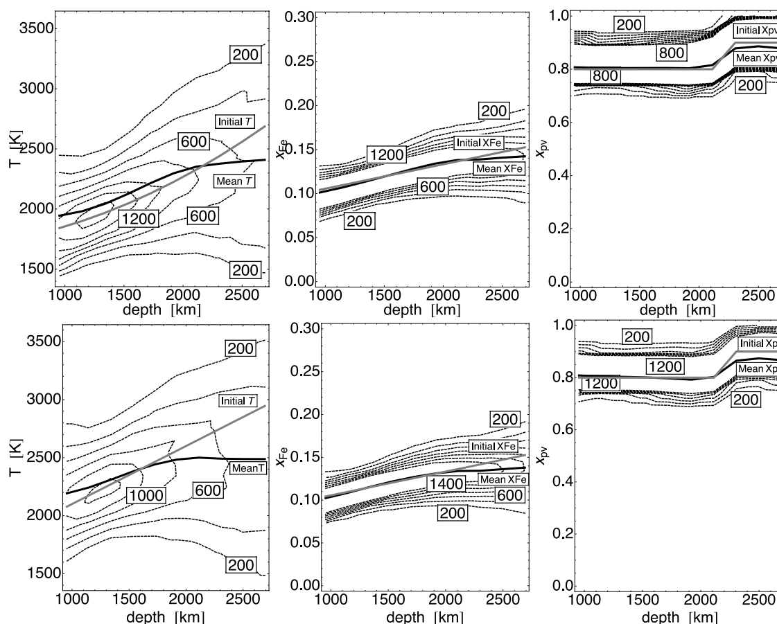
Figure 6. Results of synthetic tests for two parameter sets. (top) The geotherm is a second-order polynomial computed from Matas et al. [2007]. The temperature gradient is equal to 0.25 \text{ K km}^{-1} at 800 km depth, and temperature values are equal to 1800 K and 2800 K at 800 and 2600 km depth, respectively. (bottom) Superadiabatic geotherm with potential temperature and linear temperature gradient equal to 1600 K and 0.5 \text{ K km}^{-1} . Temperature values are equal to 2000 K and 2900 K at the top and at the bottom of the model, respectively. In both cases, the iron fraction increases linearly with depth, from 10 to 15%. The model is divided into two subregions of perovskite content equal to 80 and 90% above and below 2060 km depth. The gray curve corresponds to the initial value; the black curve represents mean values estimated by stochastic inversion of the synthetic data. Dashed curves with labels indicate the distribution of 8000 sample models at each depth. (left) Temperature; (middle) iron content; (right) perovskite fraction. Vertical axis span the range of values tested in the inversion.
