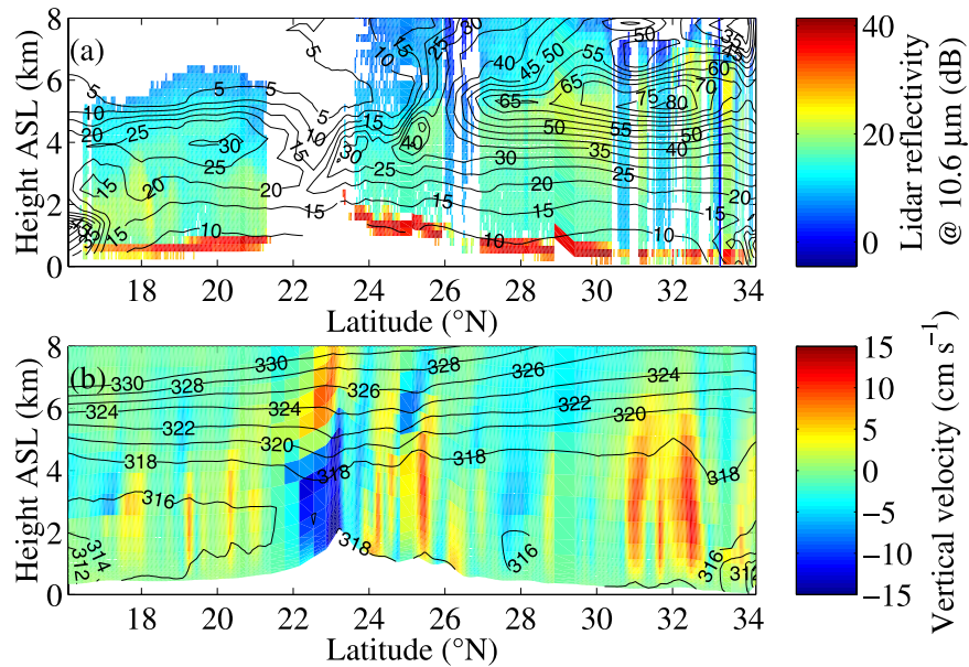
Figure 12. Vertical cross section of (a) lidar reflectivity retrieved from the WIND measurements along the leg flown by the DLR Falcon 20 between 0850 and 1235 UTC (Figure 1) and relative humidity simulated with WRF with 20-km mesh grid resolution at 1000 UTC (isocontours) and (b) simulated vertical velocity at 1000 UTC along the leg flown by the DLR Falcon 20 (color shading) and simulated isentropes (isocontours).
