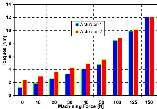
Figure 16. Actuators maximum torques with F_c ( L_c=0.06\text{m} , Traj. II)
