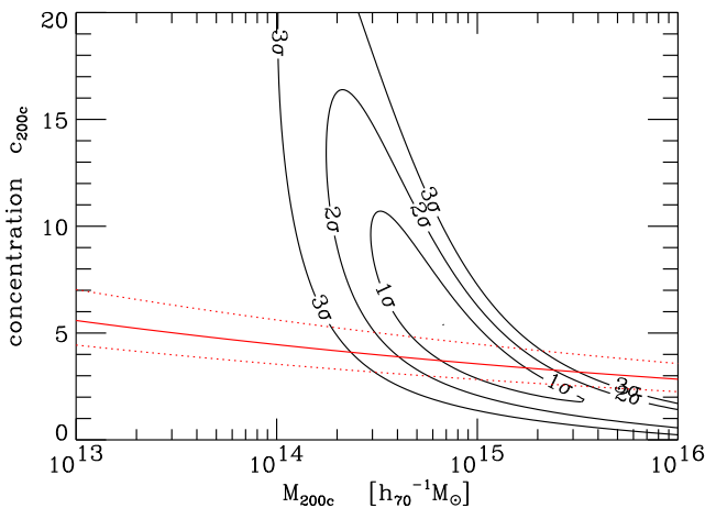
Fig. 4. M_{200c} and c_{200c} parameters constraints of the NFW density profile. The M - c relation predicted by simulation and WMAP5 cosmology (with its 1\sigma scatter) are shown in red.
