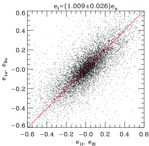
Fig. 1. Corrected ellipticities of galaxies measured in Megacam- u^* and CFH12k- I bands in the inner parts of the field. A close consistency is found with e_l = (1.009 \pm 0.026)e_u with a \sim 0.77 correlation coefficient.
