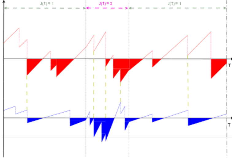
Figure 3: Two modulated risk processes with common shocks.
