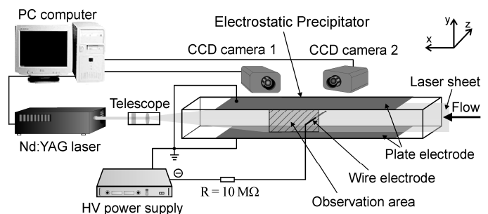
Fig. 1. Experimental set-up for 3D-PIV flow velocity field measurements in ESP.
