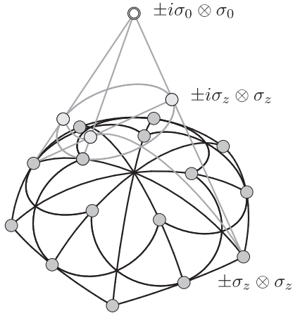
Figure 3. \mathcal{Q}_4(2) , its nucleus, and a portion of its ambient space as the geometry behind the complex two-qubit Pauli group.
