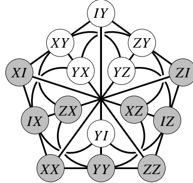
Figure 6: \mathcal{W}_3(2) and Q_3^+(2) (shaded) of the real two-qubit Pauli group. XY is a short-hand for \pm X \otimes Y , etc.
