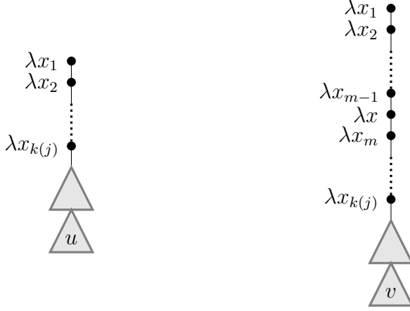
Figure 5: Terms t \in \overline{\mathcal{I}_n^{g,j}} and \varphi_n^{\mathcal{I}}(t) from Theorem 45
