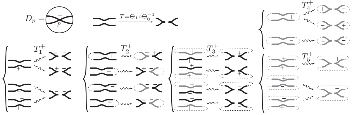
Figure 3.1: Case of a splitting at a positive double point p ( \epsilon(p) = + ).
