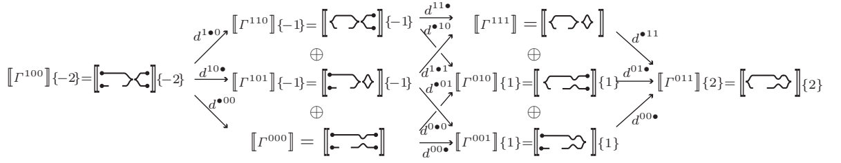
Figure 4.25: Splitting diagram of [[\Gamma]] .
