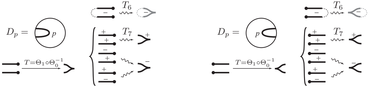
Figure 3.3: Case of a splitting at a vertical tangent point p .
