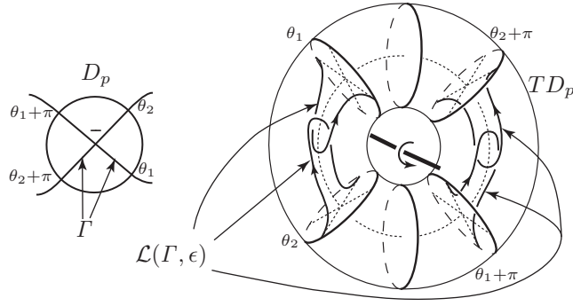
Figure 1.1: The link \mathcal{L}(\Gamma, \epsilon) over a negative double point.
