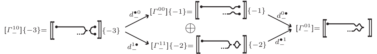
Figure 4.21: Splitting diagram for type V_- move.
