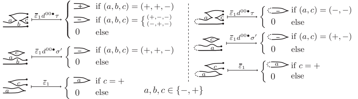
Figure 4.14: The retraction R .
