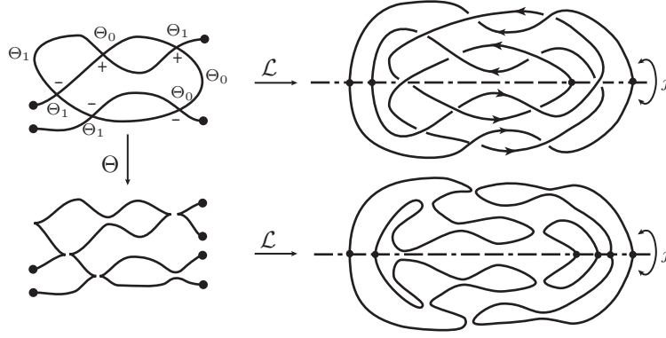
Figure 2.2: The links \mathcal{L}(\Gamma, \epsilon) and \mathcal{L}(\Theta(\Gamma, \epsilon)) , \Theta = \Theta_{1110010} .
