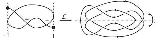
Figure 1.2: A representative OMS-divide for the strongly invertible knot 5_2 .
