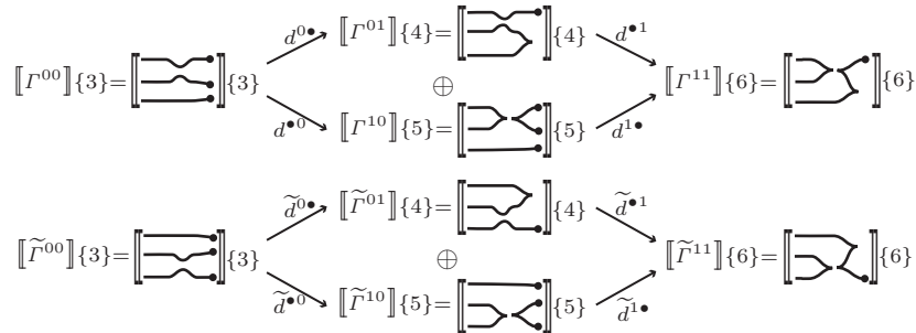
Figure 4.2: Splitting diagram for type I move.
