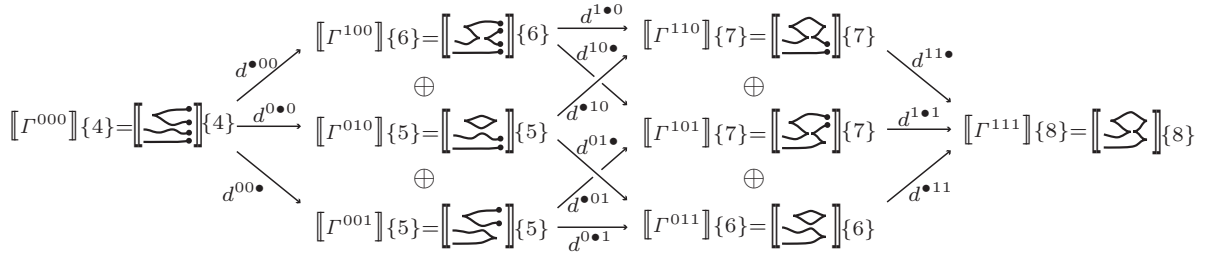
Figure 4.12: Splitting diagram of [[\Gamma]] .
