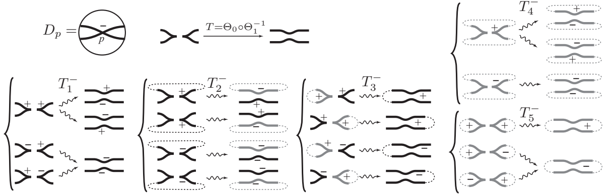
Figure 3.2: Case of a splitting at a negative double point p ( \epsilon(p) = - ).
