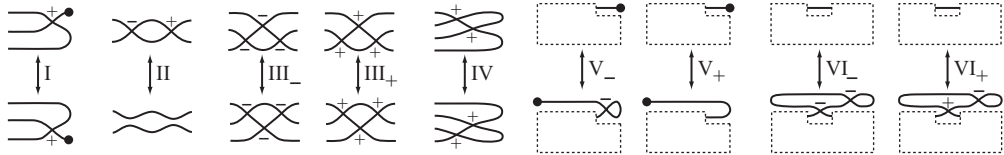
Figure 1.3: Moves of \mathcal{M} -equivalence.
