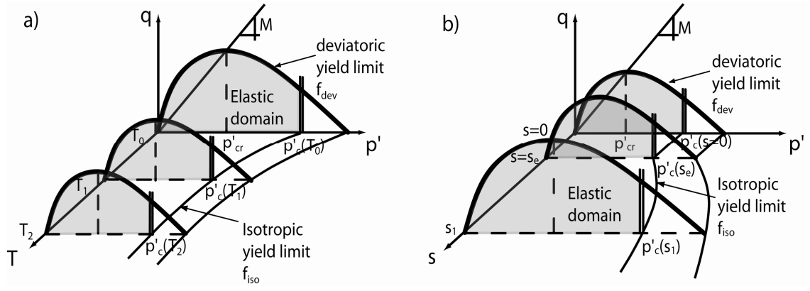
Figure 1: Effect of (a) temperature and (b) suction on the shape of coupled mechanical yield limits.
