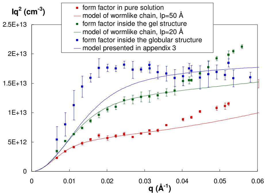
Figure 4 : Kratky plot of the three PSS form factors : Pure solution of PSS (red squares); PSS chains inside the gel structure at I = 5 \cdot 10^{-2} \text{ M} (green squares); PSS chains inside the globular structure at I = 5 \cdot 10^{-1} \text{ M} (blue squares). The continuous lines correspond to the fits. Red line : form factor of a wormlike chain ( l_p = 50 \text{ \AA} ). Green line : form factor of a wormlike chain ( l_p = 20 \text{ \AA} ). Blue line : model of a linear combination of a factor of Gaussian chains with an effective gyration radius of 85 \text{ \AA} and of a wormlike chain ( l_p = 30 \text{ \AA} ). See appendix 3 for details of the third model.
