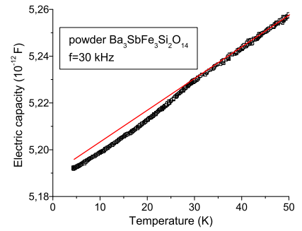
FIG. 12: Thermal variation of the electric capacity (proportional to the dielectric permittivity) of a pellet of BSFS powder. The red line is a linear extrapolation of the data above 30 K, shown to emphasize the cusp.
