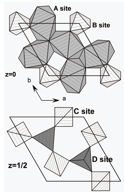
FIG. 1: Polyhedral representation of the langasite structure with its four different cation sites on two layers.
