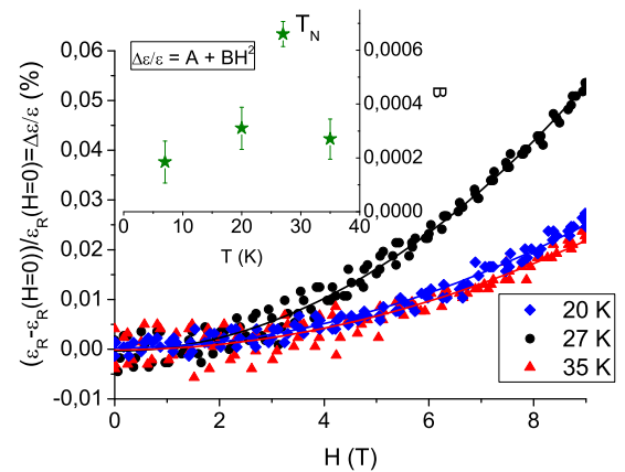
FIG. 13: Magnetic dependence of the relative variation of the BNFS single crystal dielectric permittivity, for several temperatures. Both magnetic and electric fields are applied perpendicular to the c axis. The lines are parabolic fits. The inset shows the quadratic coefficient versus temperature.
