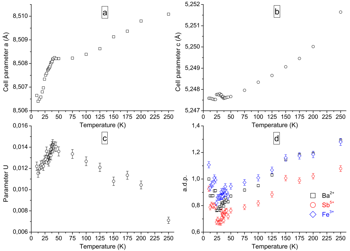
FIG. 10: Thermal variation of some refined parameters from ID31 x-ray powder diffraction data on \text{Ba}_3\text{SbFe}_3\text{Si}_2\text{O}_{14} : a) cell parameter a ( \text{\AA} ). b) cell parameter c ( \text{\AA} ). c) quadratic term U of the Gaussian peak width function. d) a.d.p.'s of \text{Ba}^{2+} , \text{Sb}^{5+} and \text{Fe}^{3+} cations.
