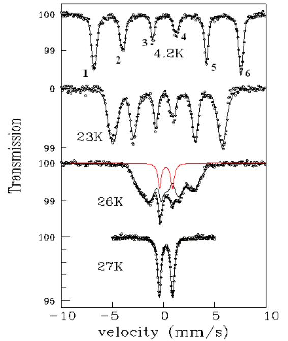
FIG. 8: ^{57}\text{Fe} Mössbauer absorption spectra in \text{Ba}_3\text{NbFe}_3\text{Si}_2\text{O}_{14} at selected temperatures. The spectra at 4.2, 23 and 26 K (circles) are fitted (black lines) to the helical magnetic structure model determined by neutron scattering. At 26 K, a quadrupolar subspectrum contribution (represented in red) overlapping the magnetic signal suggests that the magnetic transition is first order.
