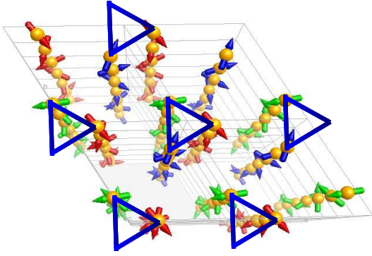
FIG. 6: Magnetic structure of the Fe-langasites: within each triangle of the (a,b) plane, the \text{Fe}^{3+} magnetic moments are rotated by 2\pi/3 from each other. The global phase factor, which cannot be determined by neutron diffraction, was arbitrary chosen equal to zero in this representation (one moment pointing towards the center of the triangles). Along the c -axis, the helix propagates with a period of 1/\tau in cell unit.
