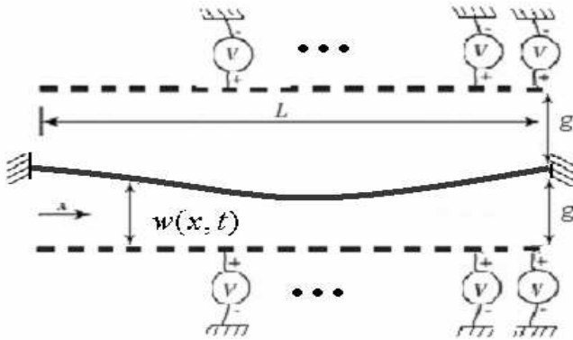
Fig. 1. The deformable microbeam surrounded with two sets of N electrodes on each side, subjected to different variant distributed voltages.
