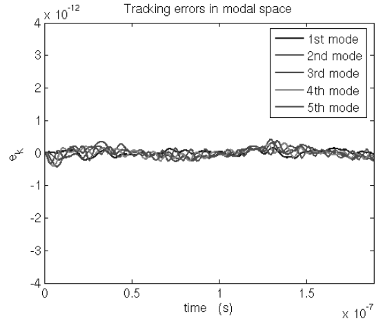
Fig. 7. The modal tracking errors coefficients for the 5 modes. One can notice that errors don't exceed the 10% of the reference coefficients.
