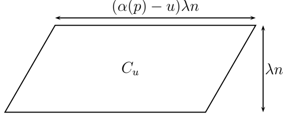
Figure 6: Structure of C_u
