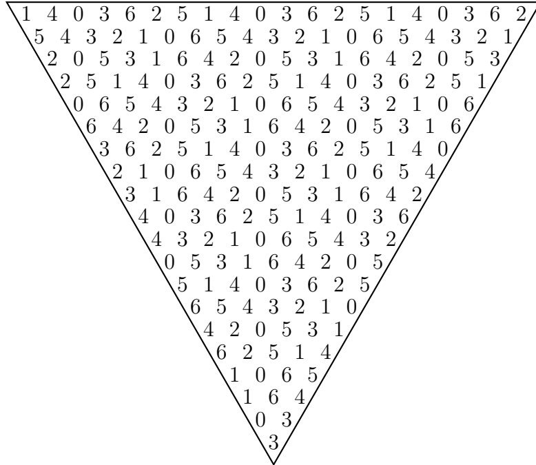
Figure 9: The Steinhaus triangle \Delta AP(1, 3, 20)
