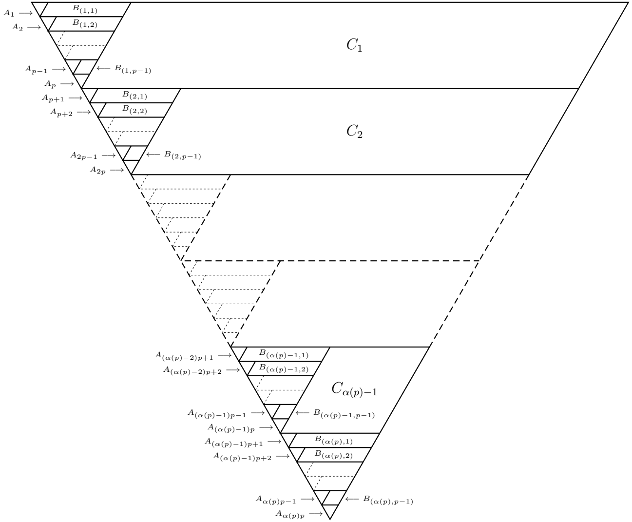
Figure 5: Structure of \Delta X
