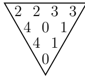
Figure 2: The Steinhaus triangle of a balanced sequence in \mathbb{Z}/5\mathbb{Z}
