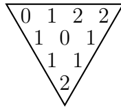
Figure 1: A Steinhaus triangle in \mathbb{Z}/3\mathbb{Z}
