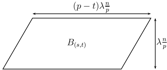
Figure 7: Structure of B_{(s,t)}
