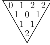
Figure 1: A Steinhaus triangle in \mathbb{Z}/3\mathbb{Z}
