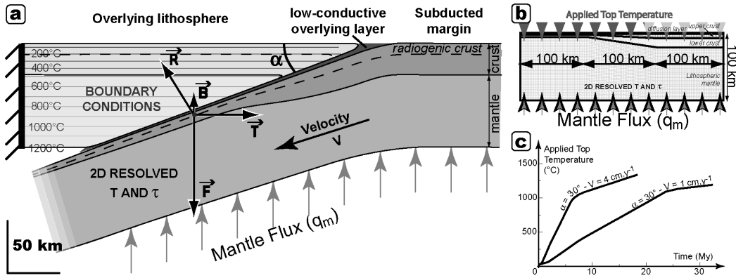
Figure 2: Model set-up. a-2D thermal model and the three forces acting on the subducted continental margin: buoyancy \vec{B} , tectonic \vec{T} and overlying weight \vec{F} forces. At equilibrium, the acting force i.e. the sum of the three previous forces, is equal to the opposite of the reaction material force: \vec{A} = -\vec{R} . See Appendix B for a detailed description of the forces and related stresses. Continental subduction is described by a dip angle \alpha and velocity V . Thermal boundary conditions are a steady-state continental geotherm in the overlying lithosphere and a mantle heat flux q_m at the base of the subducted lithosphere. The 2D model will resolve heat conduction only in the subducted lithosphere and a thin low-conductive overlying layer, which accounts for heat transport between the subducted lithosphere and the overlying lithosphere. The subducted lithosphere strength will be also calculated from the 2D temperature distribution, which evolves with the burial history. b-The geometry of the passive margin that will enter subduction is composed by three successive 100 km long domains: a thinned lithosphere with a 10 km thick crust, a transition zone where the crustal thickness progressively increases and finally, a non-thinned lithosphere with a 30 km thick continental crust. c-The applied top temperature calculated from the steady continental geotherm of the overlying lithosphere increases with burial depths, and thus time, as a function of the subduction dip angle ( \alpha ) and the velocity ( V ). See text for further details.
