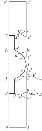
FIGURE 1. The fundamental domain for m = 13
