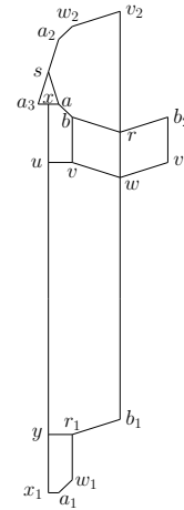
FIGURE 3. The fundamental domain for m = 10
