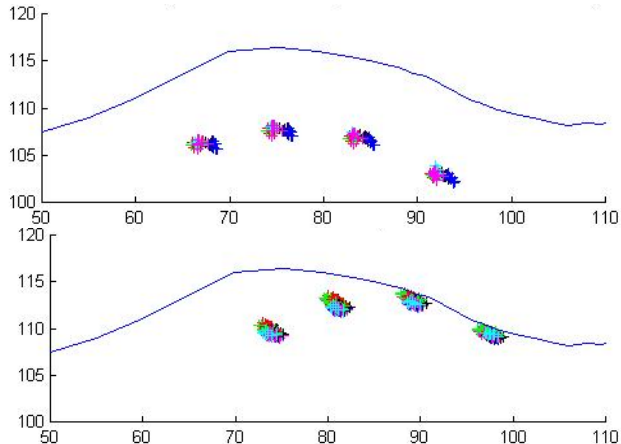
Figure 3: Node positions at target in / \text{ɔkV}_2 / sequences for the sequential planning model, where V_2 is either /i/ (green), /e (red)/, / \text{ɛ} / (magenta), / \text{œ} / (cyan), / \text{ɔ} / (black) or /a/ (black). The upper solid line represents the palate contour. Lips are on the left hand side. Top panel: Vowel / \text{ɔ} /; Bottom panel: Consonant /k/
