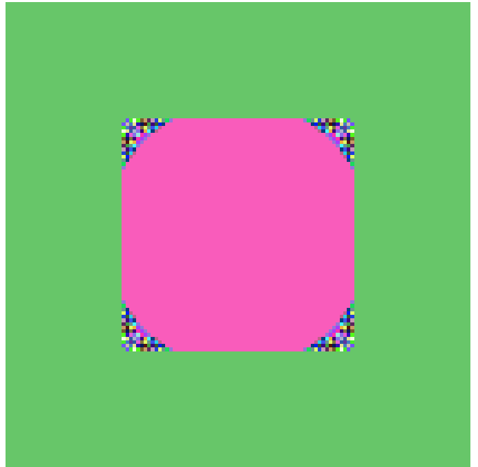
FIGURE 8. The solution of the discrete BV problem using the upwind definition (17) in “false color” ( 128 \times 128 ).
