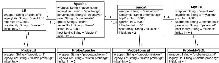
Fig. 3. Architecture schema for J2EE
