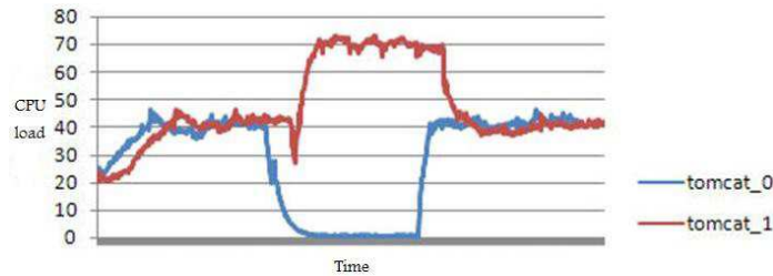
Fig. 2. Automatic restart of a Tomcat server on software fault
