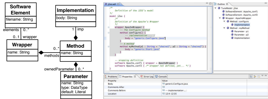
Fig. 7. The Wrapping Description Language
