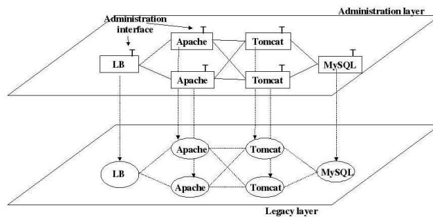
Fig. 1. Management layer for the J2EE application
