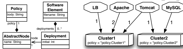
Fig. 8. The Deployment Description Language
