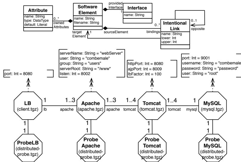
Fig. 6. The Configuration Description Language
