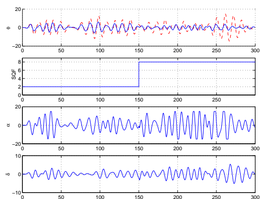
Figure 6. Variation of SQF during simulation. Closed loop (solid), open loop (dashed).
