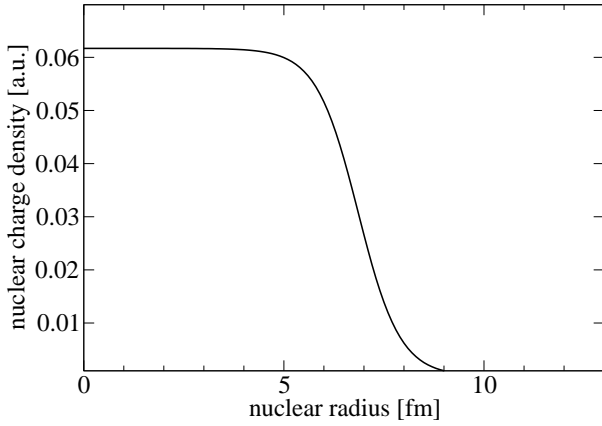
FIG. 1: Nuclear charge density \rho [a.u.] as function of the nuclear radius r [fm], using a two-parameter Fermi distribution for the ^{225}_{88}\text{Ra} nucleus.
