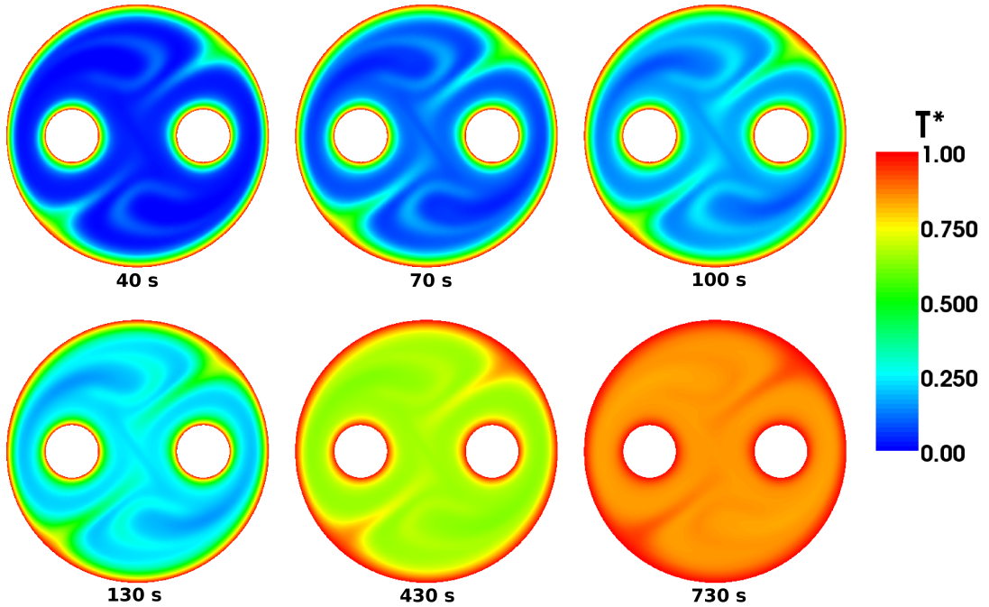
Figure 13: Snapshots showing the evolution of the temperature field towards a strange eigenmode for stirring configuration 2 and modulation period \tau = 30 s .
