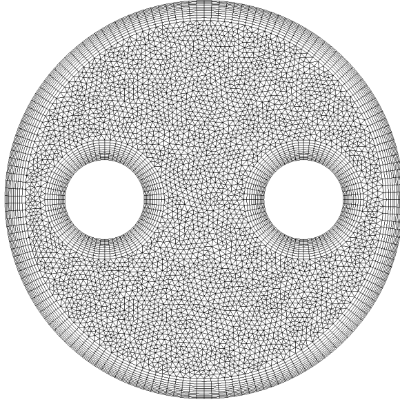
Figure 4: Computational mesh of the mixer.
