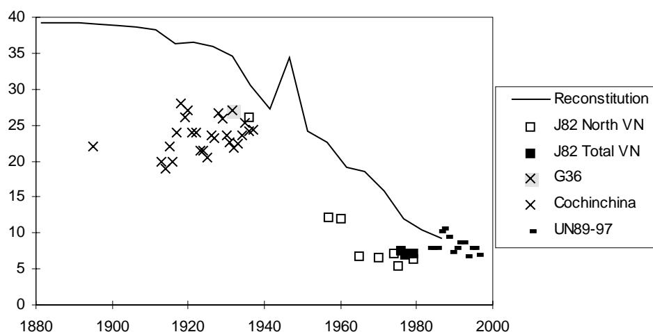
Figure 15 Reconstituted Crude Death Rates and other Crude Death Rate estimates: United Nations 1989 and 1997 (UN89;97); Jones 1982 North and total Vietnam (J82 N-VN and J82 VN); Gourou 1936 (G36); Vietnam Annaires 1897-1937 (Cochinchina)
