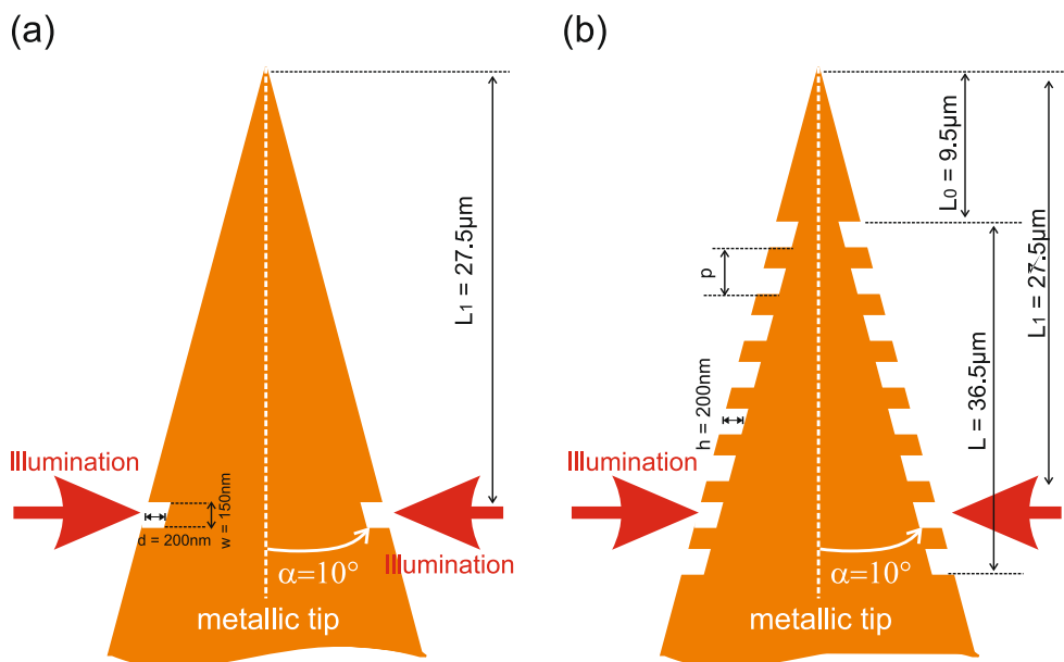
Fig. 3 Theoretical model of the structured tip with a groove (a) or with a finite grating (b)
