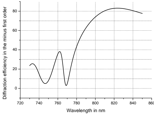
Figure 1 : -1^{\text{st}} diffraction efficiency spectrum in a standard dielectric mirror based corrugated silica layer with n(\text{SiO}_2) = 1.48 , n(\text{HfO}_2) = 2.118 , groove depth = 650 nm, groove width = 342 nm and 193 nm unetched silica layer.
