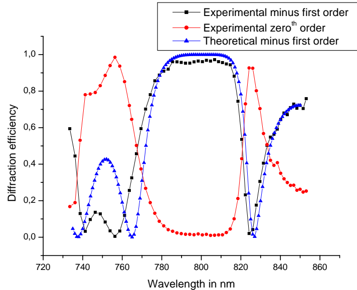
Figure 6 : Theoretical and experimental -1^{\text{st}} order diffraction efficiency and experimental 0^{\text{th}} order reflection spectra in a \text{HfO}_2/\text{SiO}_2 multilayer based grating of 536 nm period under 60^\circ incidence of the TE polarization.
