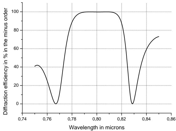
Figure 3 : Theoretical diffraction efficiency versus wavelength in a multielectric mirror based pair of low and high index layers.
