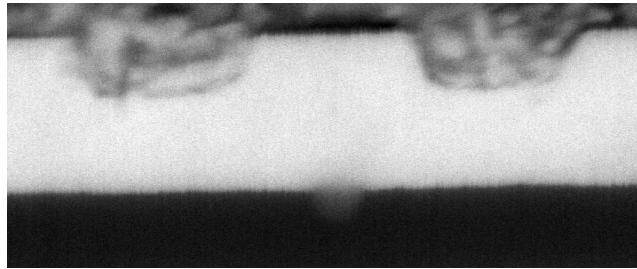
Figure 4 : SEM Picture of the corrugated hafnia layer cross section.
