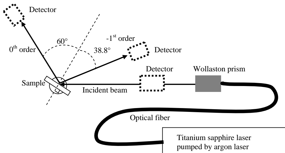
Figure 5 : Sketch of the measurement setup
