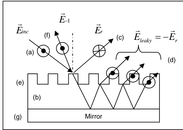
Figure 2 : Leaky mode excitation (d) enabling the cancellation of the 0 th reflected order (c).
