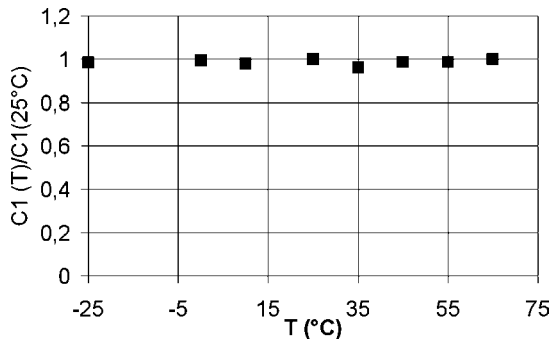
Fig. 13. Capacitance of capacitor A_1 as a function of temperature.
