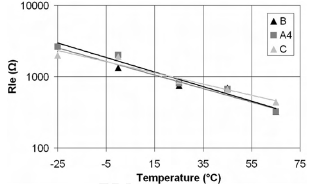
Fig. 21. Resistance R_{le} versus temperature for components A_4 , B, and C.
